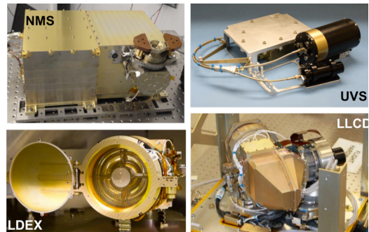
LADEE's payload consists of three science instruments and a technology demonstration.
